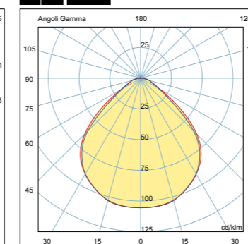
MORSE wall/ceiling 2x... FLT G5
