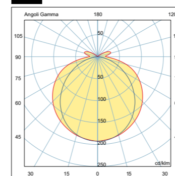
SKY LIGHT super 14 2x80W
