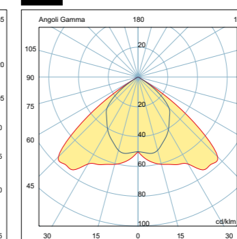
SKY LIGHT super 15 1x49W
