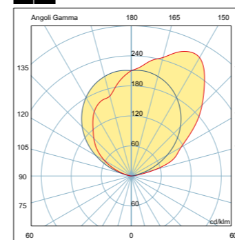
FUTURA wall compact 1x55W
