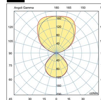
MORSE suspension 2x... FLT G5
