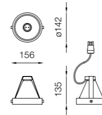
MH G12 spot
