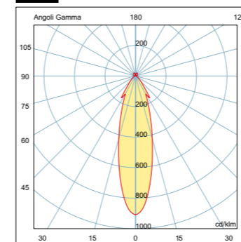
TAM TAM suspension diffuser 1x...MH-G12
