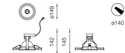
MH G12 spot
