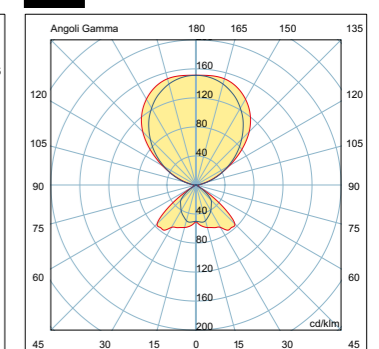
SKY LIGHT super 15B 1x49W+2x80W
