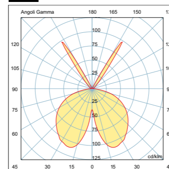
TAM TAM suspension reflecta 1x...MH-G12
