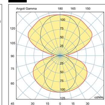
SKY LIGHT super 14B 2x80W
