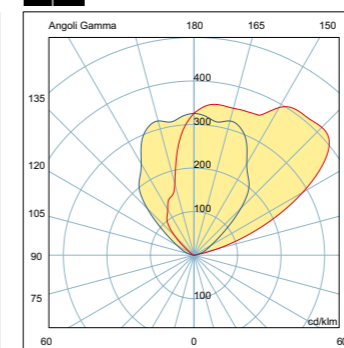
FUTURA wall compact 1x ... MH-Rx7S
