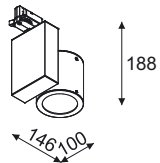
T096B2Sm ...color1 ...power [W] / D[°]
